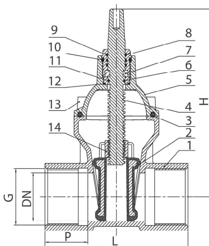
DN40/DN50
